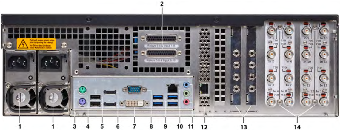
Figure 3: Rear view G-ST 6000+ G2
