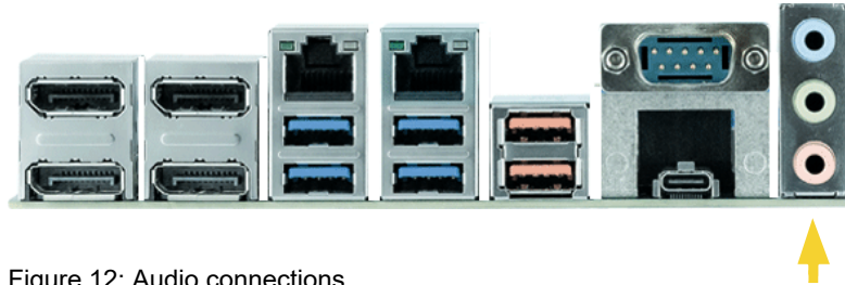
Figure 12: Audio connections
