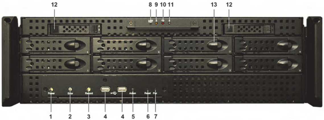
Figure 2: Front view without cover
