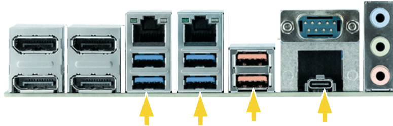
Figura 8: conexiones 4x USB 3.2 (GEN1) 2x USB 3.2 (GEN2) 1x USB-C 3.2 (GEN2)
