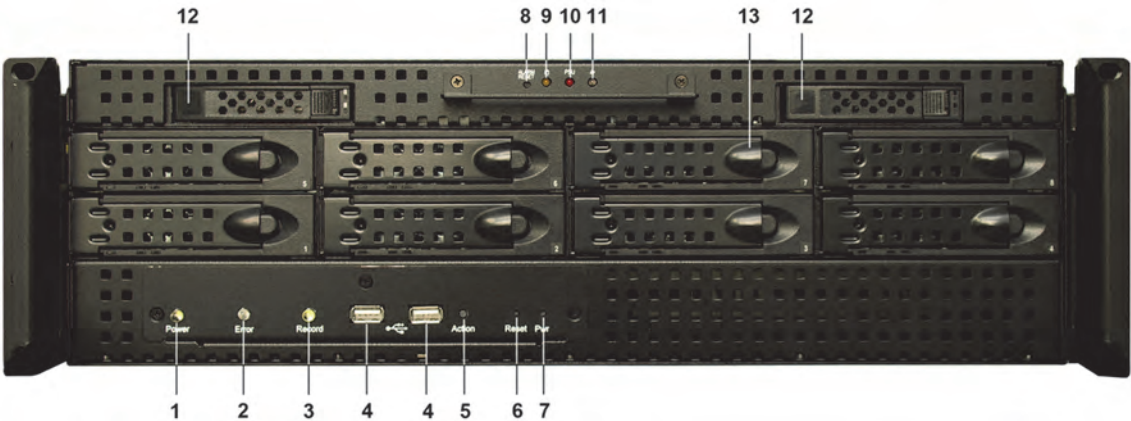
Figure 1: Front view
