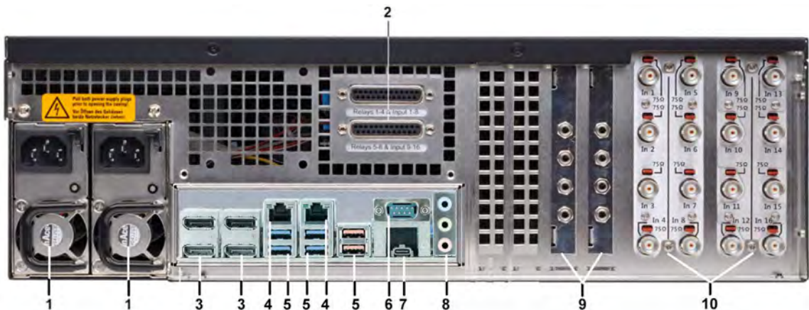
Figure 3: Rear view G-ST 6000+ G3
