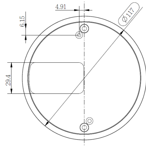
Dimensions adapter plate
