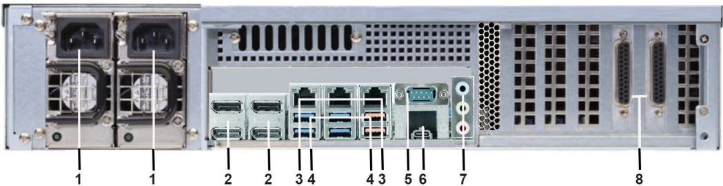
Figure: Rear view G-ST 8000+G3/2U
